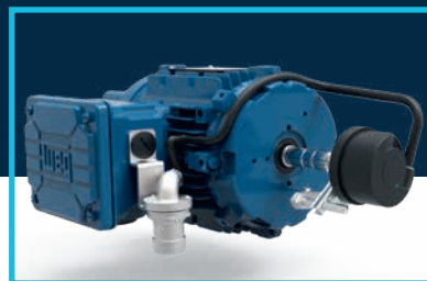
Incremental encoder (forced ventilation)
